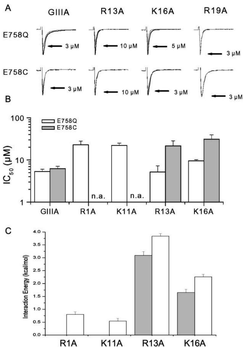
FIGURE 5 Interactions of E758 with R1, K11, R13, K16, and R19. (A) Representative Na + currents through E758Q (top panels) and E758C (bottom panels) channels recorded in the absence and presence of WT, R13A, K16A, and R19A GIIIA \mu -CTX as indicated. (B) Bar graphs summarizing the IC 50 s of E758Q (open bars) and E758C (solid bars) channels for block by WT \mu -CTX GIIIA and the derivatives R1A, K11A, R13A, K16A, and R19A. The IC 50 for block of both E758Q and E758C channels by R19A could not be determined; n.a. denotes not available. (C) Interaction (coupling) energies ( \Delta\Delta G ) of E758Q (open bars) and E758C (solid bars) channels with R1A, K11A, R13A, and K16A as estimated from the experimental IC 50 s in (B). Both E758Q and E758C interact most strongly with R13A followed by K16A but there is a relatively weak coupling of E758Q with R1A and K11A.
