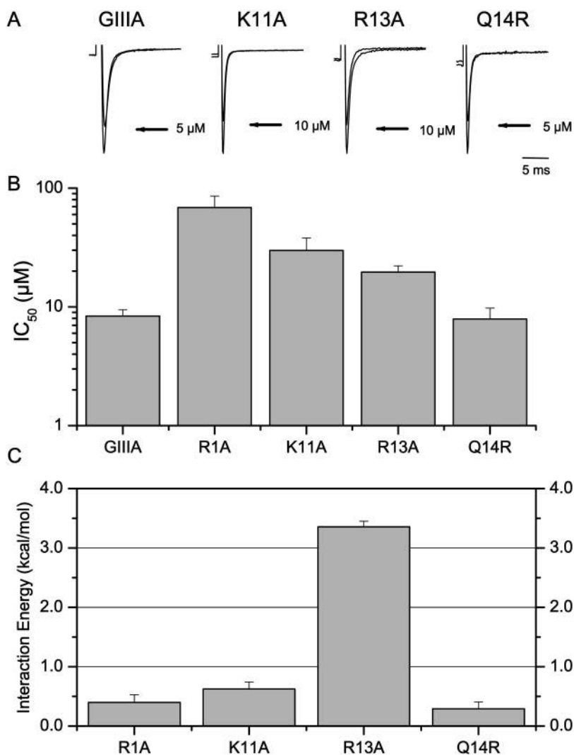
FIGURE 3 Interactions of Y401K with R1A, K11A, R13A, and Q14R. (A) Representative Na^+ currents through Y401K channels recorded in the absence and presence of WT \mu -CTX G111A and its derivatives K11A, R13A, and Q14R as indicated. (B) Bar graphs summarizing the half-blocking concentrations ( IC_{50} ) for block of Y401K channels by WT, R1A, K11A, R13A, and Q14R \mu -CTX. (C) \Delta\Delta G s for the interactions of Y401K with the same toxins as in parts A and B. Y401K was strongly coupled to R13A but not to R1A, K11A, and Q14R.
