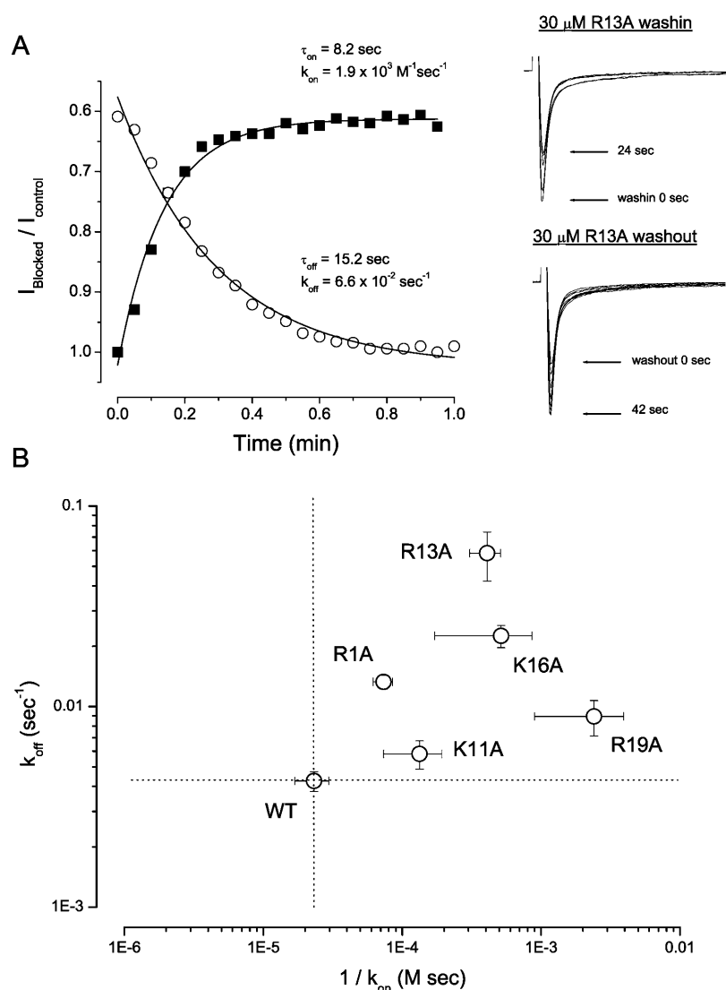
FIGURE 2 Kinetic analysis of block by mutant \mu -CTX derivatives. (A) Left Panel: Time courses of onset and offset of R13A (30 \mu M) block of WT \mu 1 channels during toxin wash in (solid squares) and wash out (open circles). Normalized peak sodium currents elicited by depolarization to -10 mV from a holding potential of -100 mV were plotted versus time. Data were fitted with a mono-exponential function to estimate \tau_{on} and \tau_{off} for toxin binding and unbinding respectively. The equations used for deriving k_{on} and k_{off} from \tau_{on} and \tau_{off} have been previously described (Li et al., 2000). Right Panel: Representative records of \mu 1 currents elicited during wash in (top) and wash out (bottom) of R13A (30 \mu M). Sweeps (15 msec duration) shown were separated by 6-s intervals for clarity. (B) Logarithmic plot of the dissociation rate constants ( k_{off} ) versus the reciprocal of the association rate constants ( k_{on} ). The horizontal and vertical dotted lines respectively represent the levels of 1/k_{on} and k_{off} for the WT channels. All mutant toxins studied (except K11A) had substantial effects on both k_{on} and k_{off} (see text for details). The largest effects on k_{on} and k_{off} were found with R19A and R13A, respectively.
